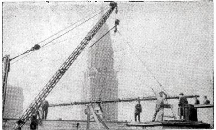
TELEVISION stopped traffic in mid-town New York last week when not-so-blase Manhattanites paused to gape as a six-bay super turnstile RCA television antenna was hoisted to the roof of the 36-floor, Daily News Bldg., where it will be installed for WPIX, "New York Daily News" video station. First installation of this new antenna—TF6A—in New York, the WPIX bat-wing will soar 754 feet above the street. It and the transmitter are scheduled to be completed in May, and WPIX is due to go on the air June 15.
